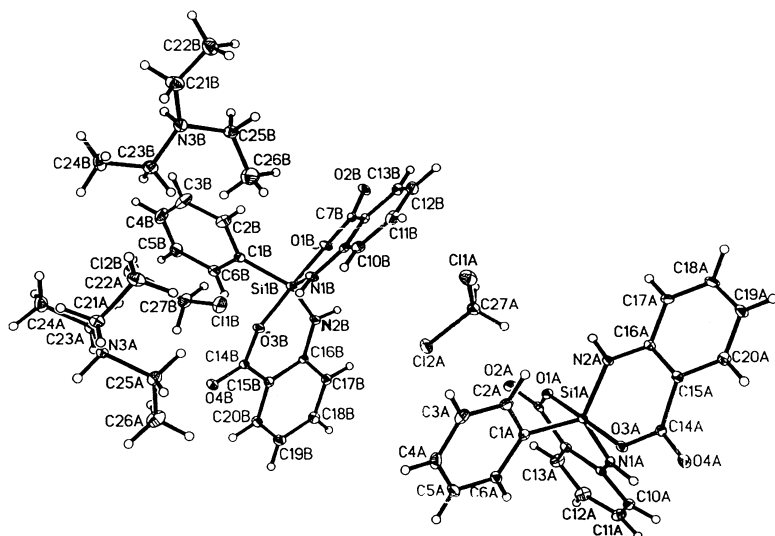
FIGURE 1 Crystal structure of 1 \cdot \text{CH}_2\text{Cl}_2 (ORTEP plot with probability level 30%), showing atomic labeling scheme. The two crystallographically independent molecules presented in a single crystal are shown with the solvent ( \text{CH}_2\text{Cl}_2 ) molecules.
